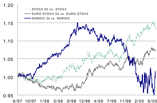
Relative Performance
